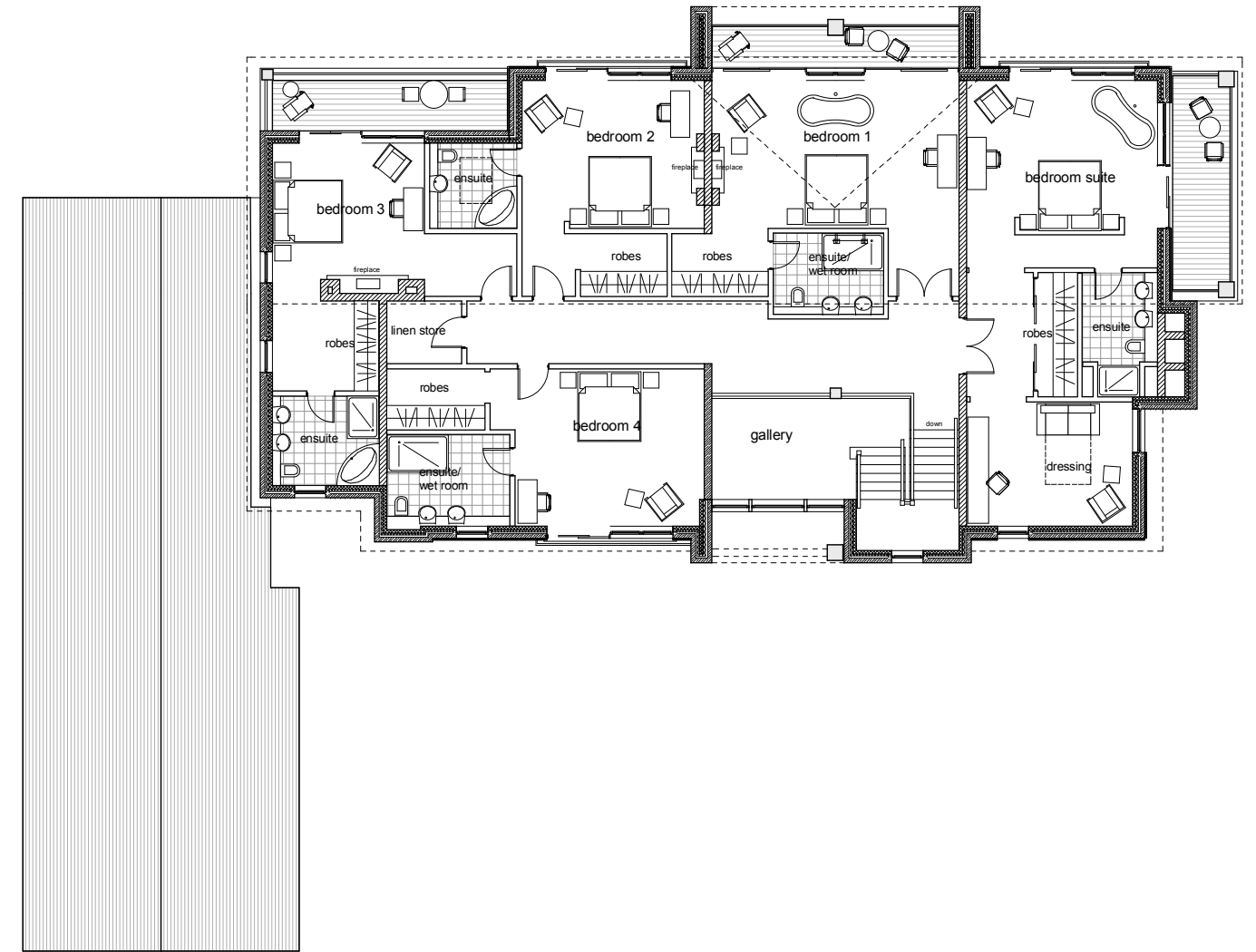
first floor layout 1:100
